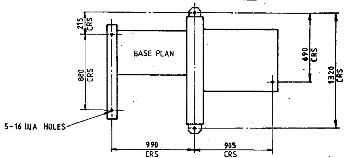
FOUNDATION PLAN FOR CP12
