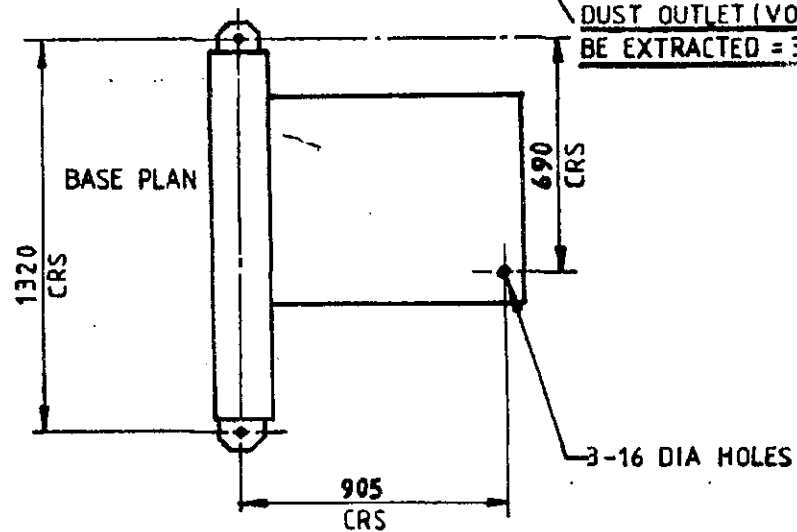
FOUNDATION PLAN FOR CP12/D
