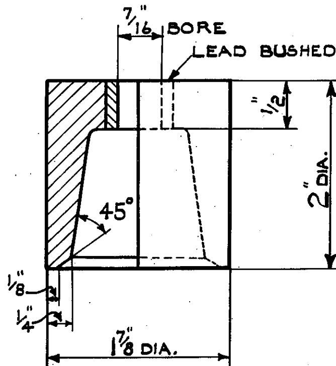
White Bauxilite Vitrified Cup Wheel Ref. UGW. 152.
