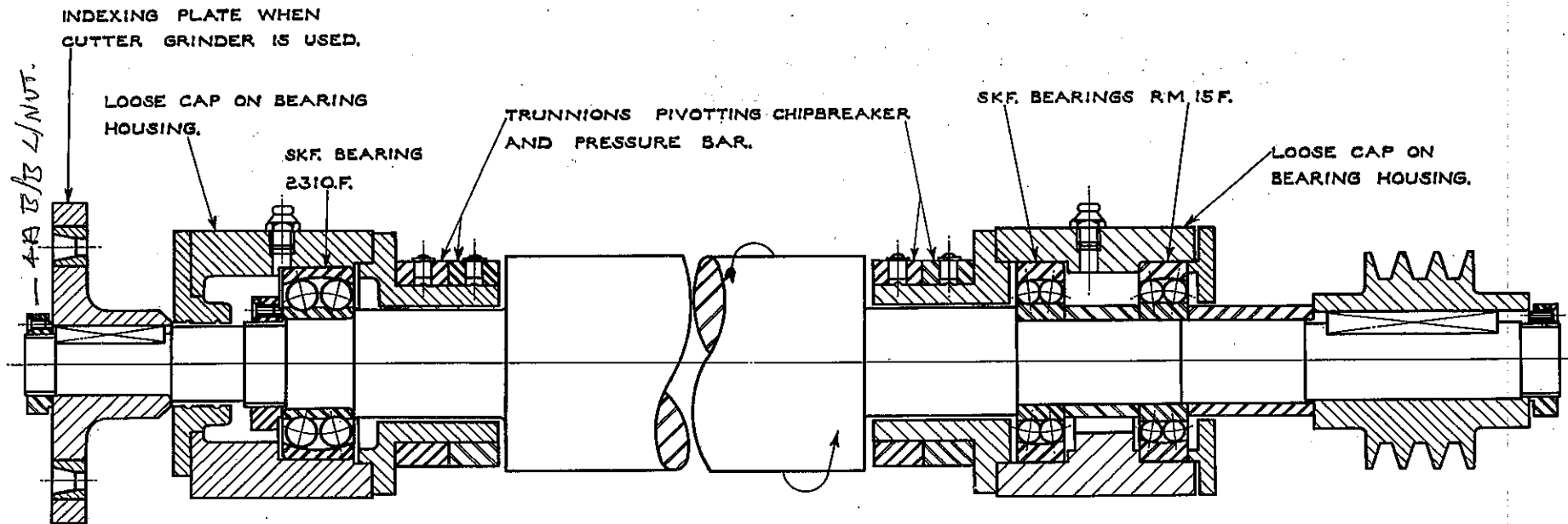
FIG. 5. ARRANGEMENT OF CUTTERBLOCK SPINDLE.
