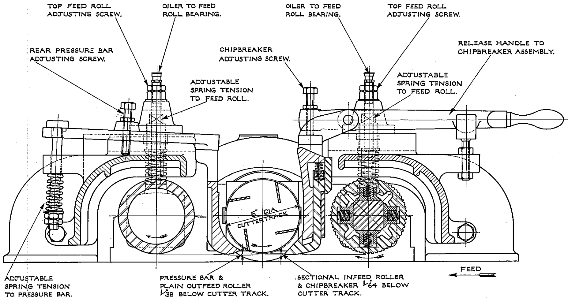
ADJUSTMENT OF FEED ROLLERS AND TOP PRESSURES.
