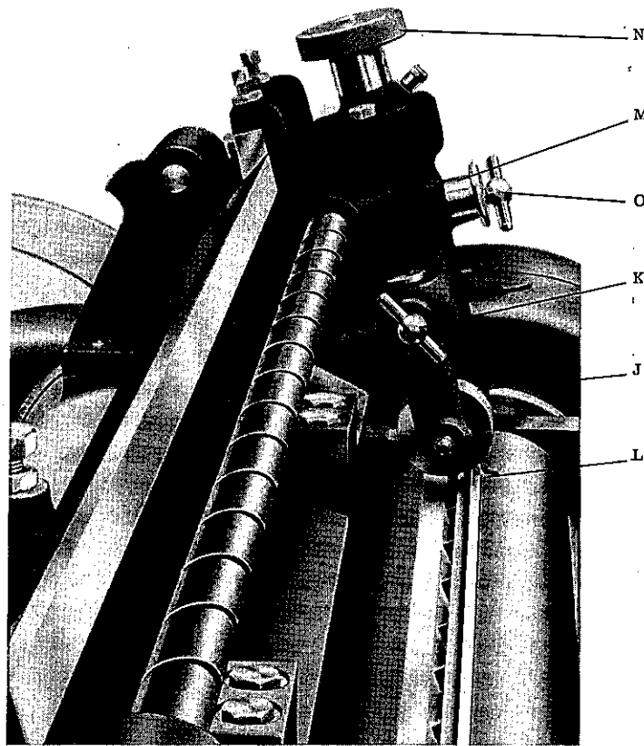
Fig. 8. KNIFE SETTING AND JOINTING DEVICE
